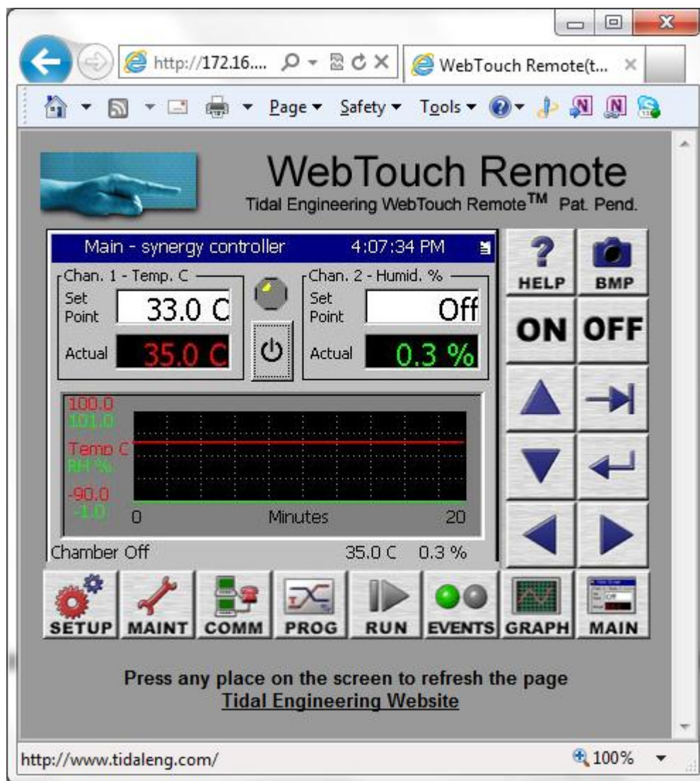
Figure 1 Synergy Controller Webtouch Remote Interface
